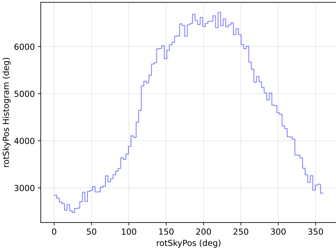
too_elab_r8_d3_ugrizy_v3.4_10yrs All sky r band: rotSkyPos Histogram
