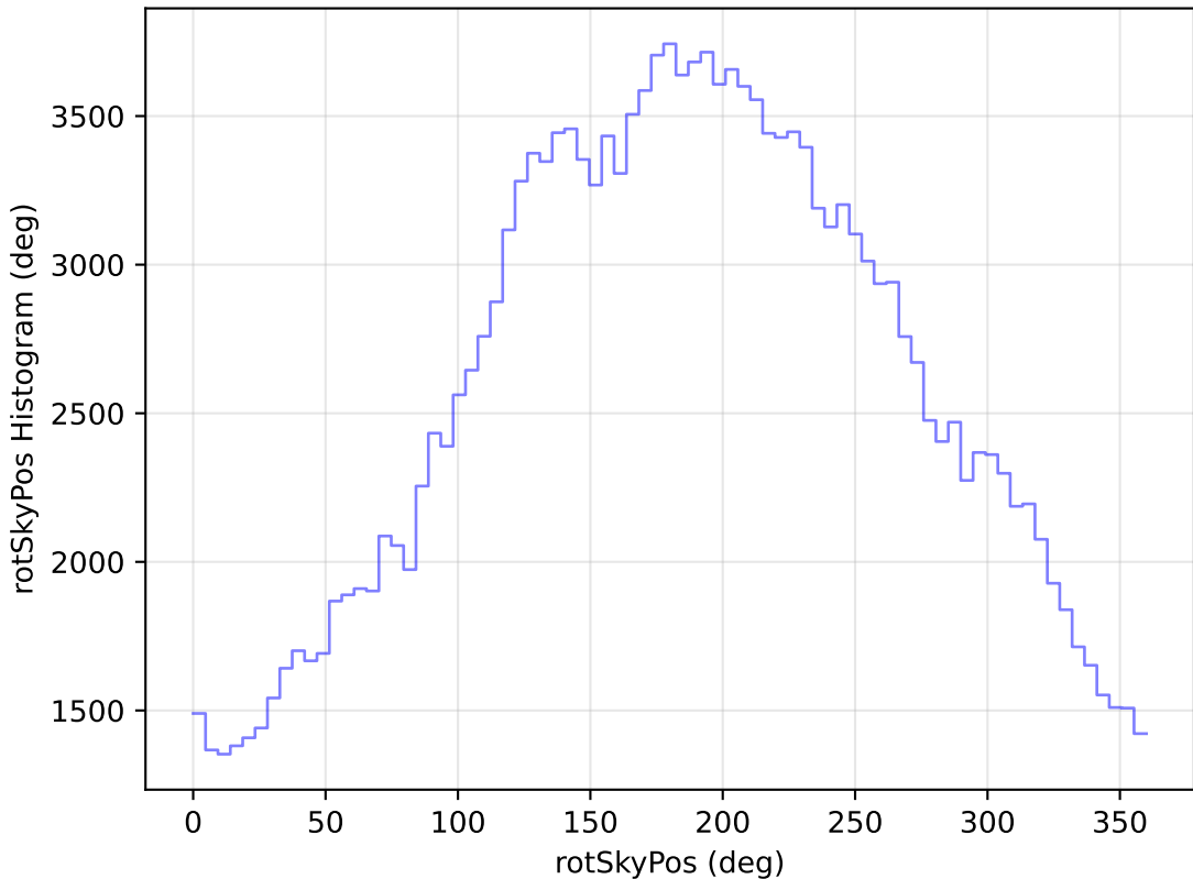
too_elab_r8_d3_ugrizy_v3.4_10yrs All sky g band: rotSkyPos Histogram
