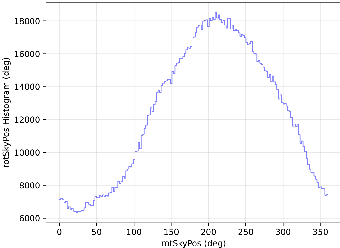
too_elab_r8_d3_ugrizy_v3.4_10yrs All sky all bands: rotSkyPos Histogram
