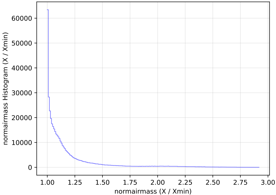
too_elab_r8_d3_ugrizy_v3.4_10yrs WFD z band: normairmass Histogram
