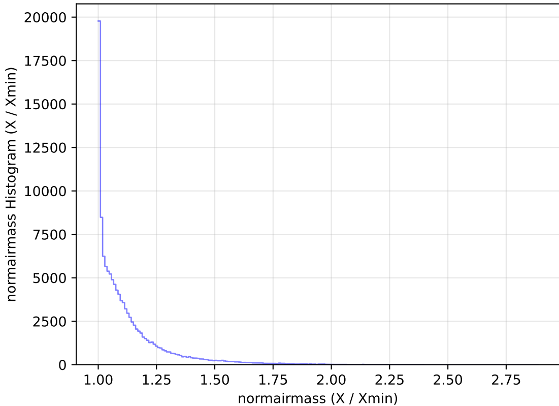
too_elab_r8_d3_ugrizy_v3.4_10yrs WFD u band: normairmass Histogram
