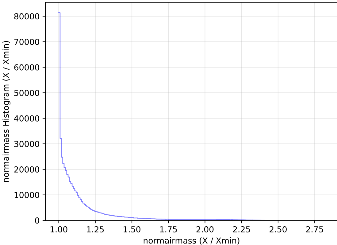
too_elab_r8_d3_ugrizy_v3.4_10yrs WFD r band: normairmass Histogram
