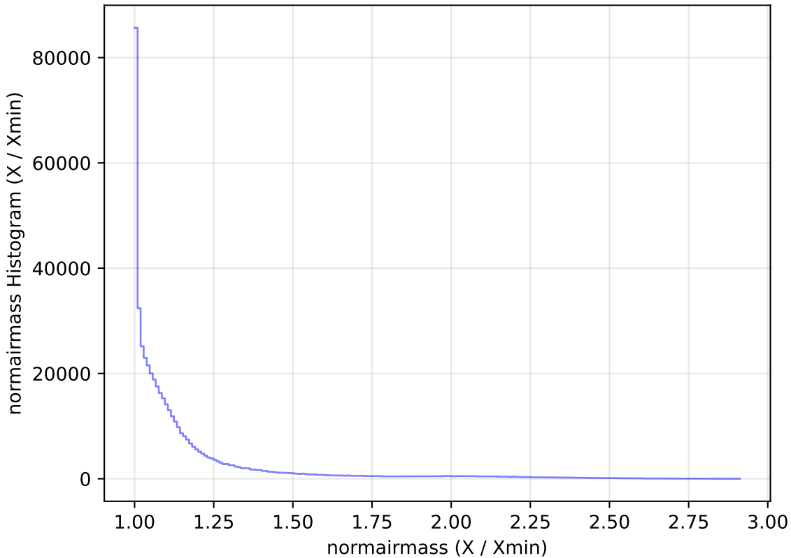
too_elab_r8_d3_ugrizy_v3.4_10yrs WFD i band: normairmass Histogram
