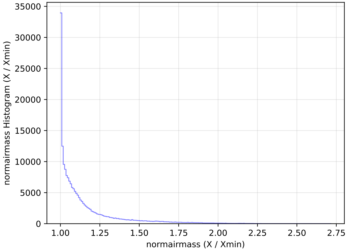
too_elab_r8_d3_ugrizy_v3.4_10yrs WFD g band: normairmass Histogram
