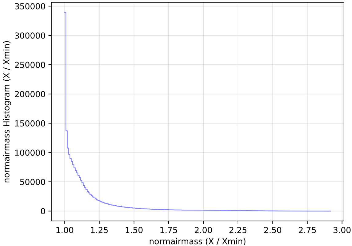
too_elab_r8_d3_ugrizy_v3.4_10yrs WFD all bands: normairmass Histogram
