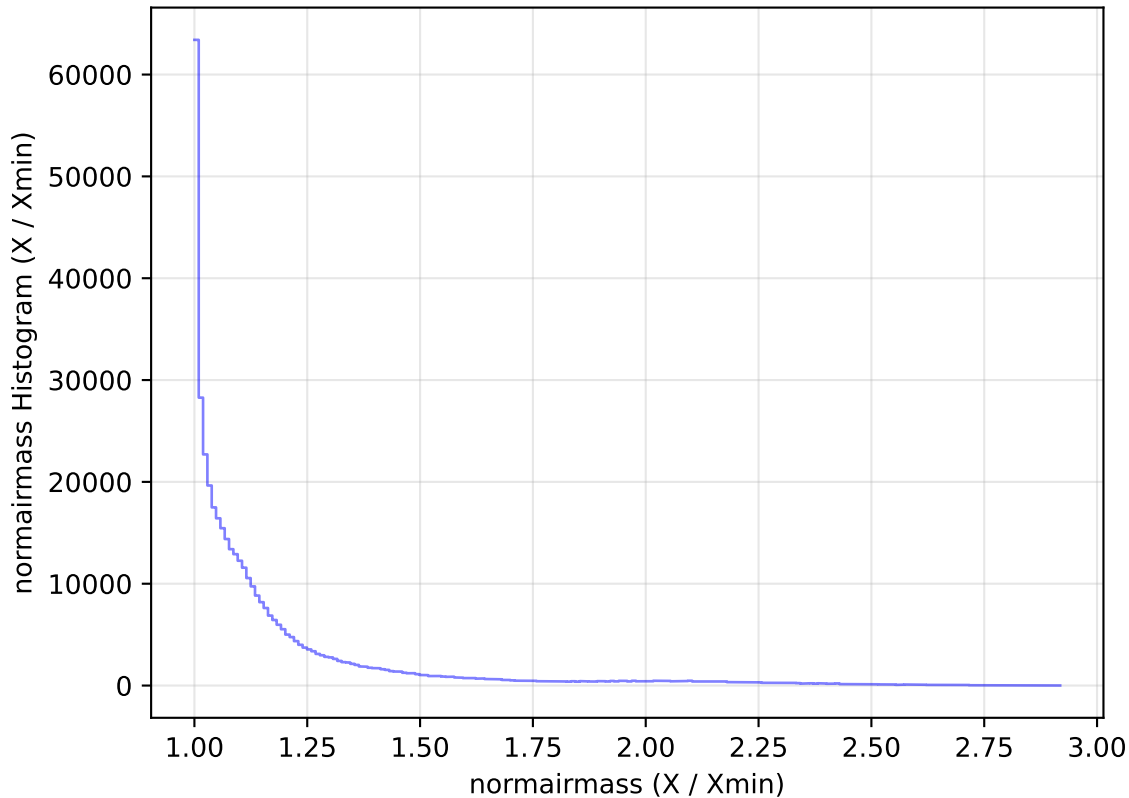
too_elab_r8_d3_ugrizy_v3.4_10yrs All sky z band: normairmass Histogram
