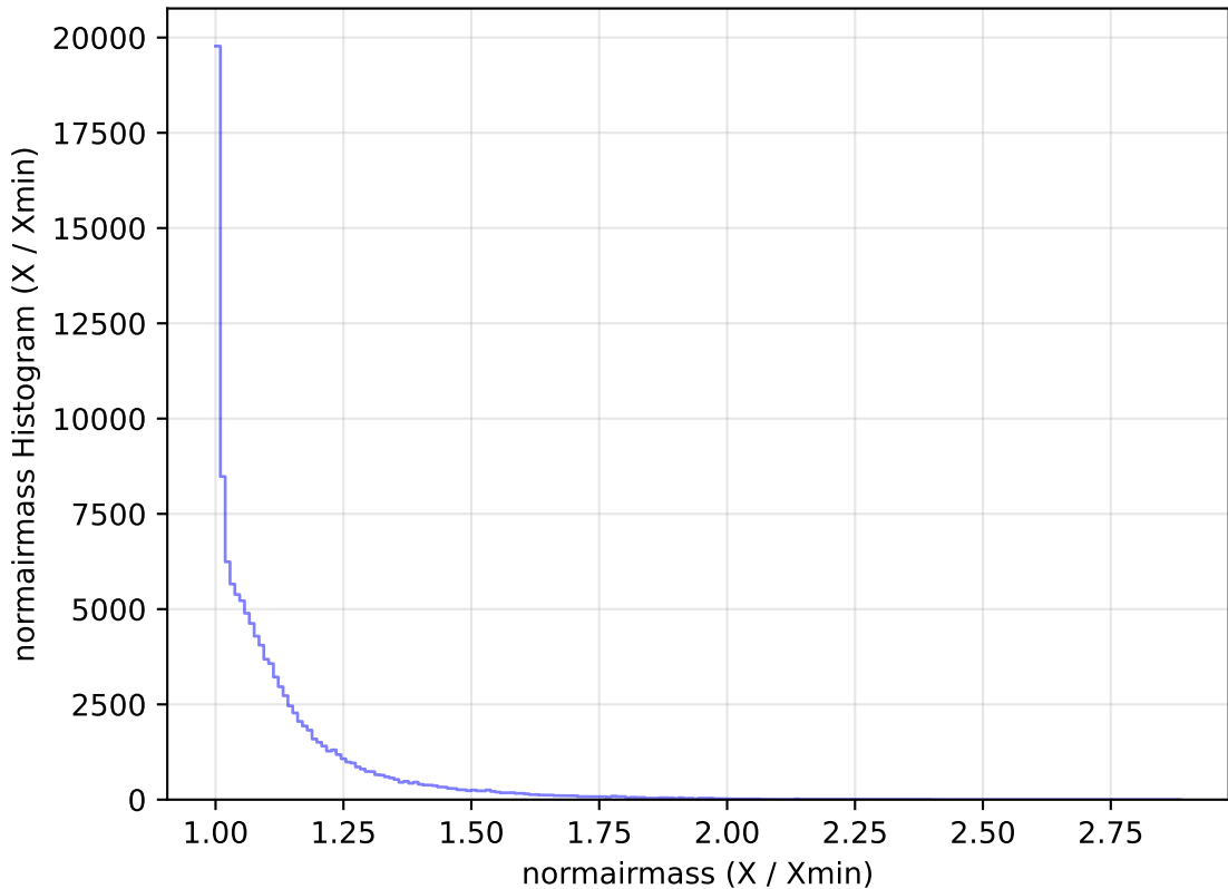
too_elab_r8_d3_ugrizy_v3.4_10yrs All sky u band: normairmass Histogram
