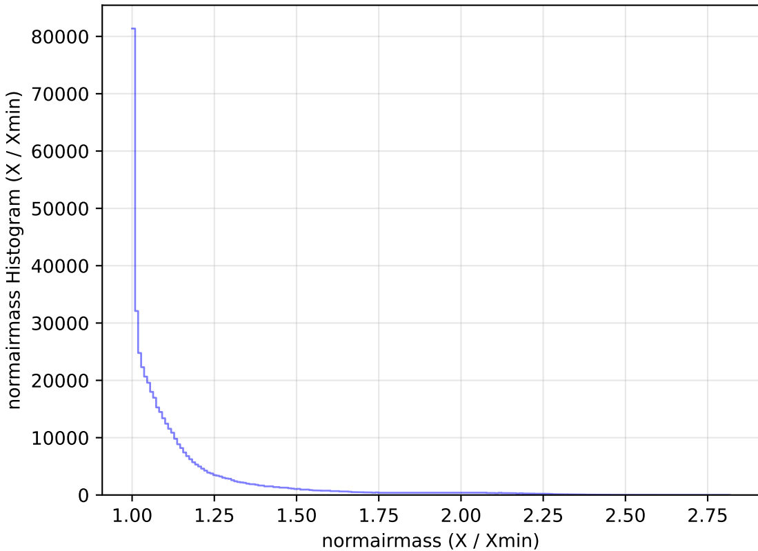
too_elab_r8_d3_ugrizy_v3.4_10yrs All sky r band: normairmass Histogram
