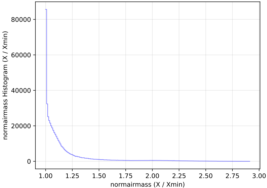
too_elab_r8_d3_ugrizy_v3.4_10yrs All sky i band: normairmass Histogram
