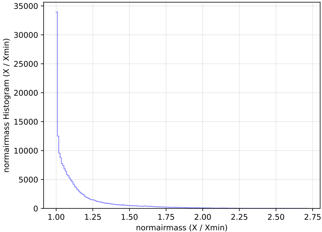
too_elab_r8_d3_ugrizy_v3.4_10yrs All sky g band: normairmass Histogram
