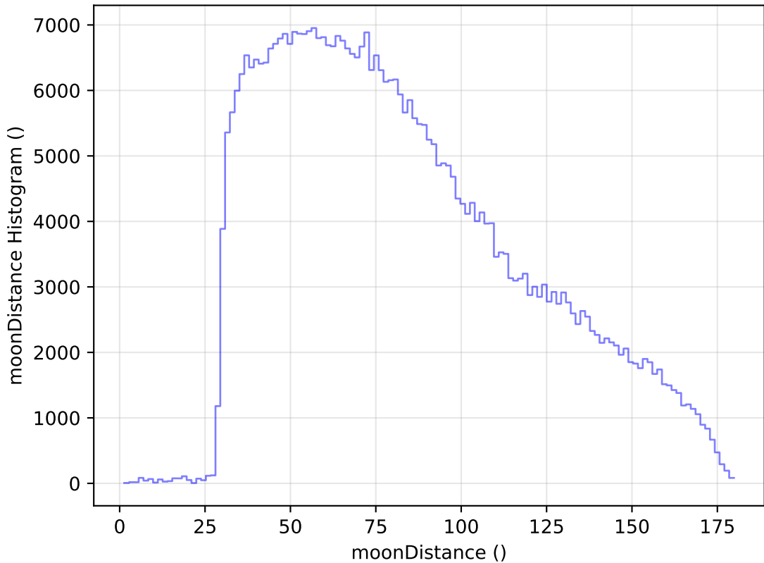
too_elab_r8_d3_ugrizy_v3.4_10yrs WFD z band: moonDistance Histogram
