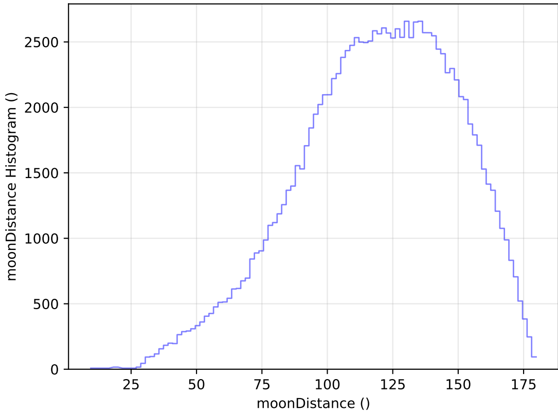
too_elab_r8_d3_ugrizy_v3.4_10yrs WFD u band: moonDistance Histogram
