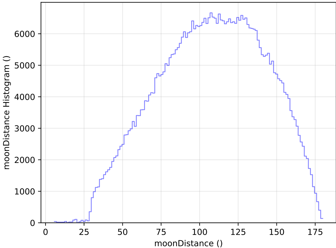
too_elab_r8_d3_ugrizy_v3.4_10yrs WFD r band: moonDistance Histogram
