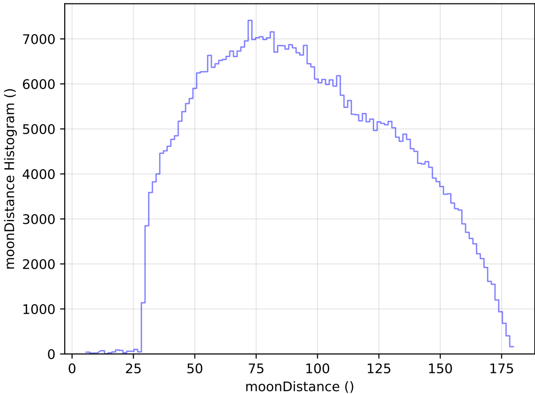
too_elab_r8_d3_ugrizy_v3.4_10yrs WFD i band: moonDistance Histogram
