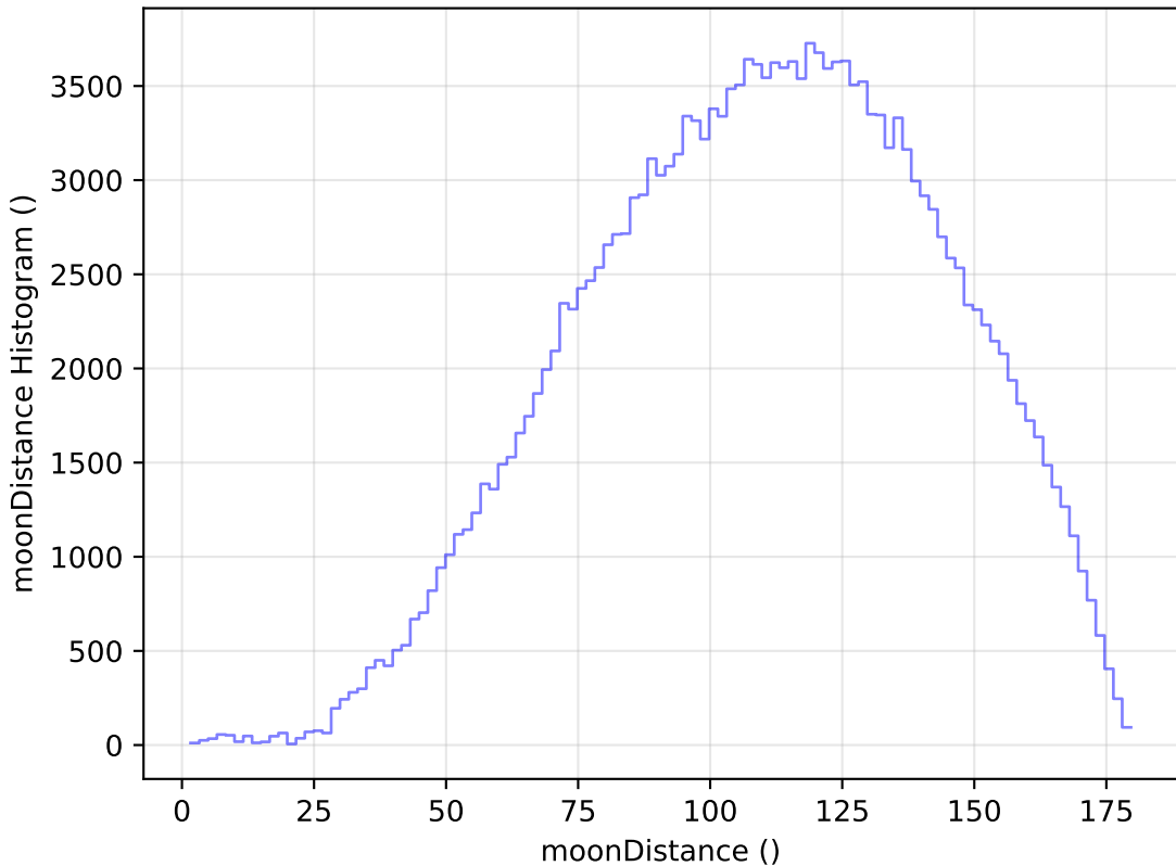
too_elab_r8_d3_ugrizy_v3.4_10yrs WFD g band: moonDistance Histogram
