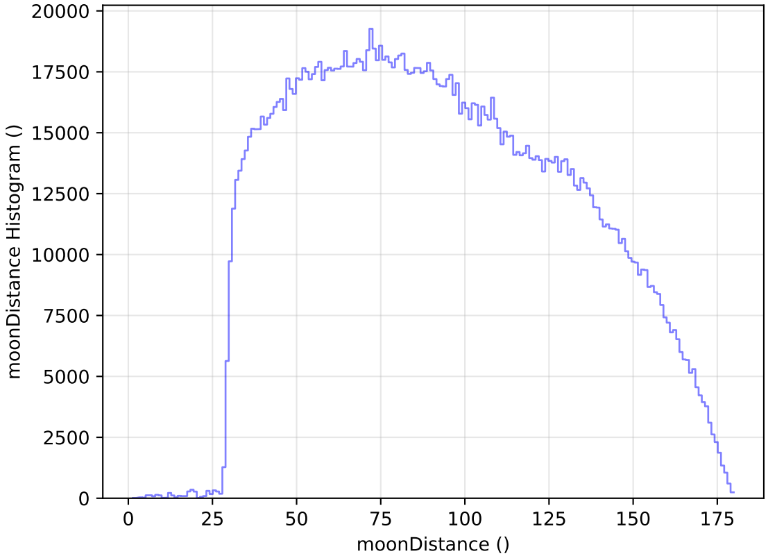
too_elab_r8_d3_ugrizy_v3.4_10yrs WFD all bands: moonDistance Histogram
