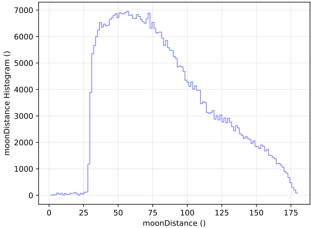
too_elab_r8_d3_ugrizy_v3.4_10yrs All sky z band: moonDistance Histogram
