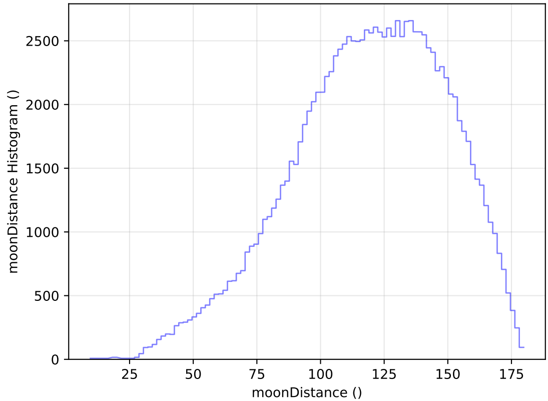
too_elab_r8_d3_ugrizy_v3.4_10yrs All sky u band: moonDistance Histogram
