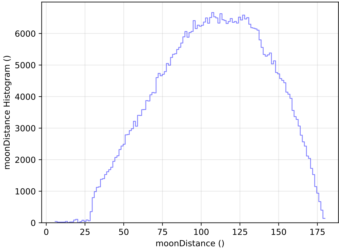
too_elab_r8_d3_ugrizy_v3.4_10yrs All sky r band: moonDistance Histogram
