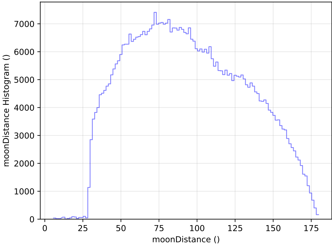
too_elab_r8_d3_ugrizy_v3.4_10yrs All sky i band: moonDistance Histogram
