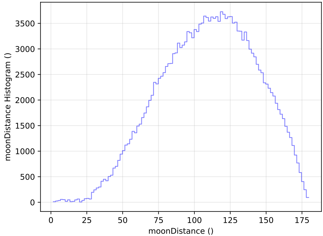
too_elab_r8_d3_ugrizy_v3.4_10yrs All sky g band: moonDistance Histogram
