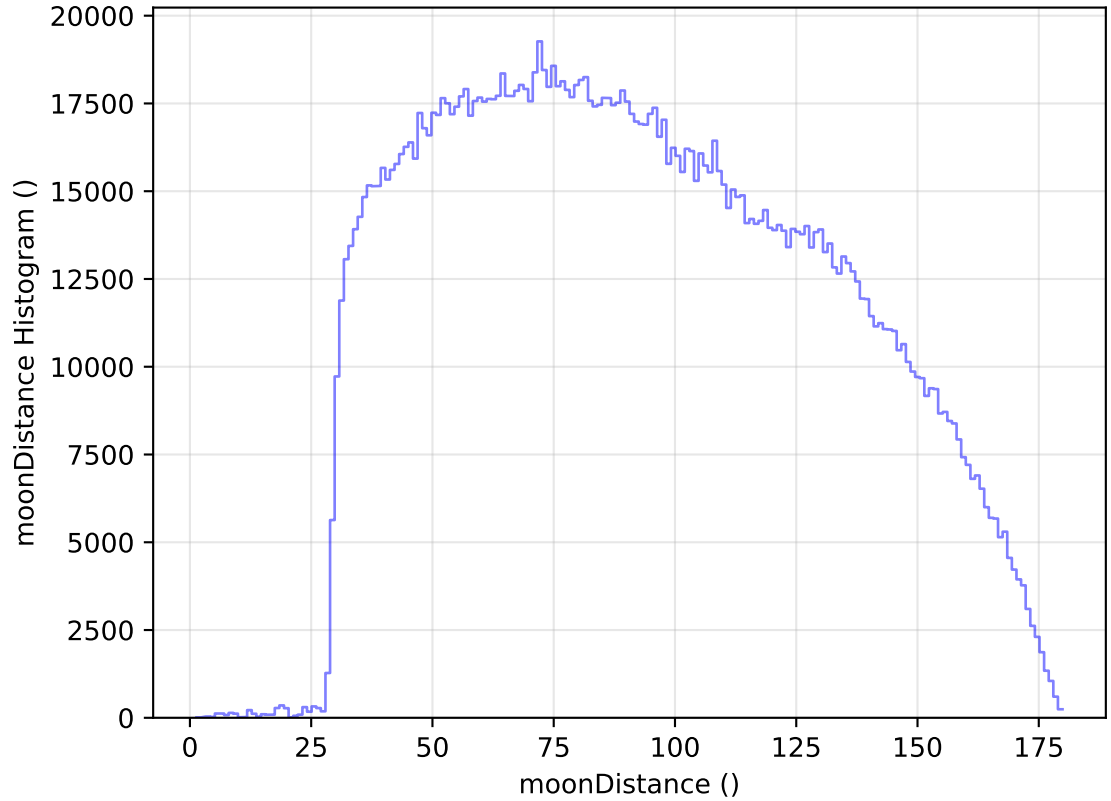
too_elab_r8_d3_ugrizy_v3.4_10yrs All sky all bands: moonDistance Histogram
