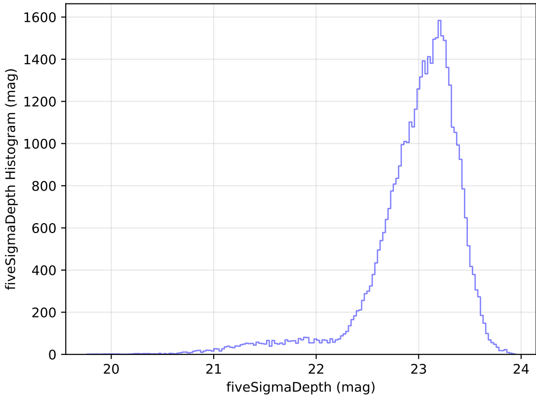
too_elab_r8_d3_ugrizy_v3.4_10yrs Yr 1 z band: fiveSigmaDepth Histogram
