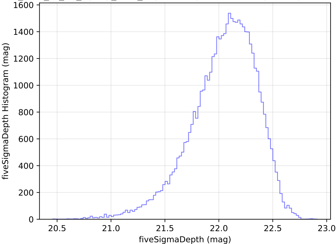
too_elab_r8_d3_ugrizy_v3.4_10yrs Yr 1 y band: fiveSigmaDepth Histogram
