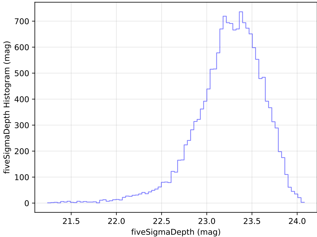
too_elab_r8_d3_ugrizy_v3.4_10yrs Yr 1 u band: fiveSigmaDepth Histogram
