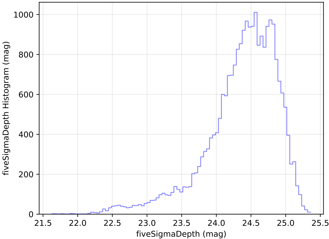
too_elab_r8_d3_ugrizy_v3.4_10yrs Yr 1 g band: fiveSigmaDepth Histogram
