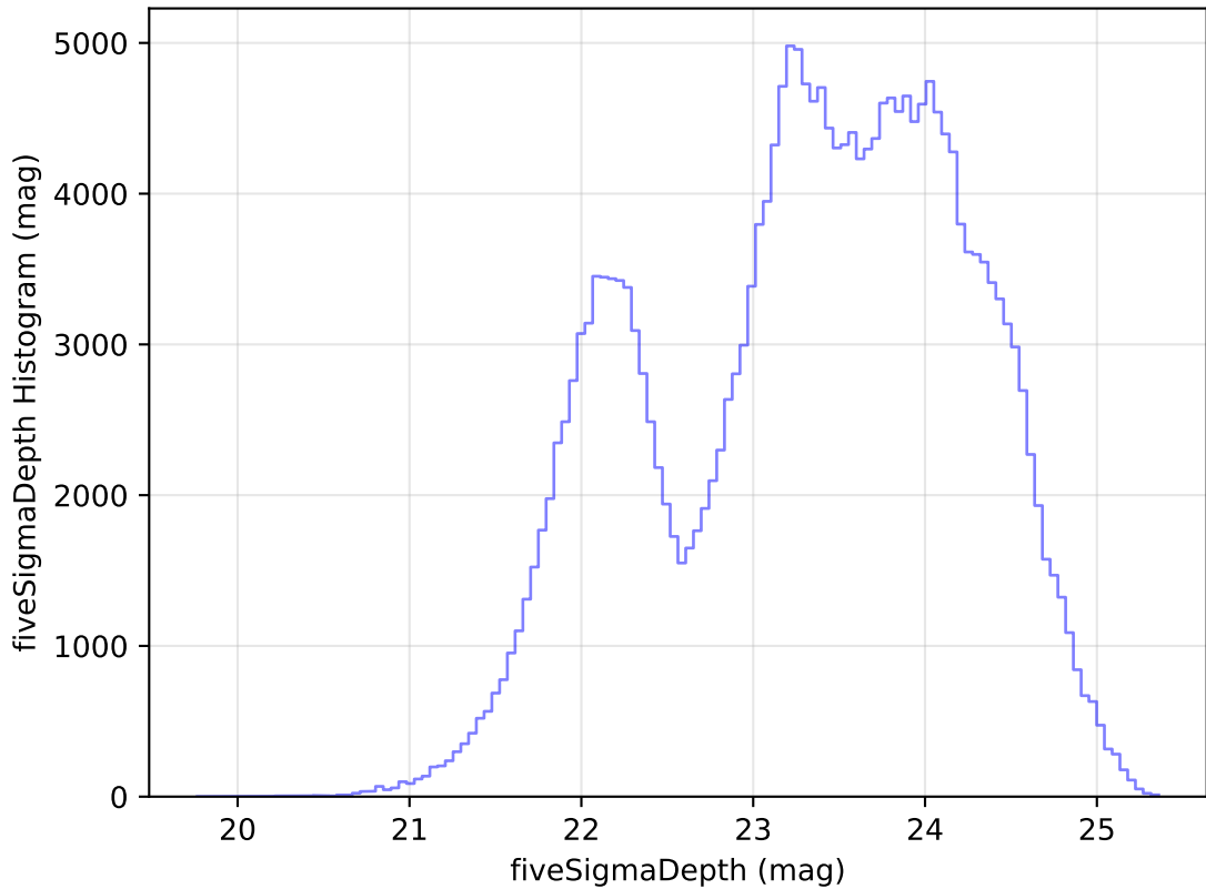
too_elab_r8_d3_ugrizy_v3.4_10yrs Yr 1 all bands: fiveSigmaDepth Histogram
