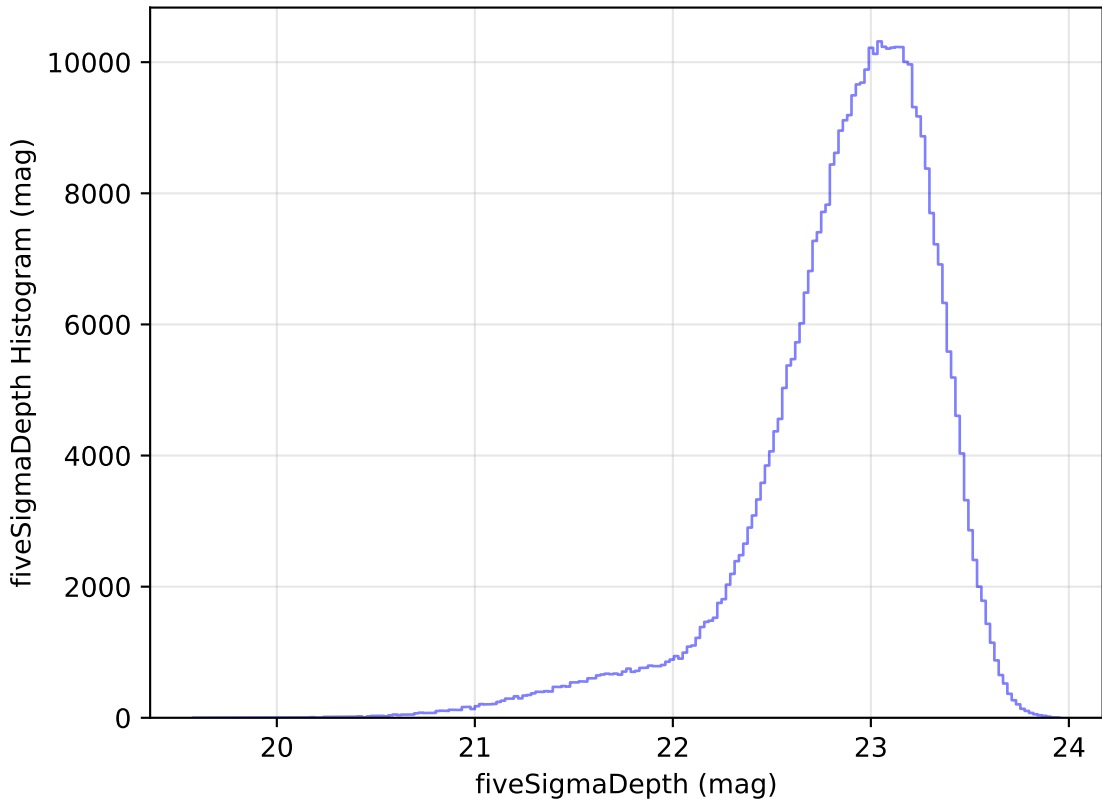
too_elab_r8_d3_ugrizy_v3.4_10yrs WFD z band: fiveSigmaDepth Histogram
