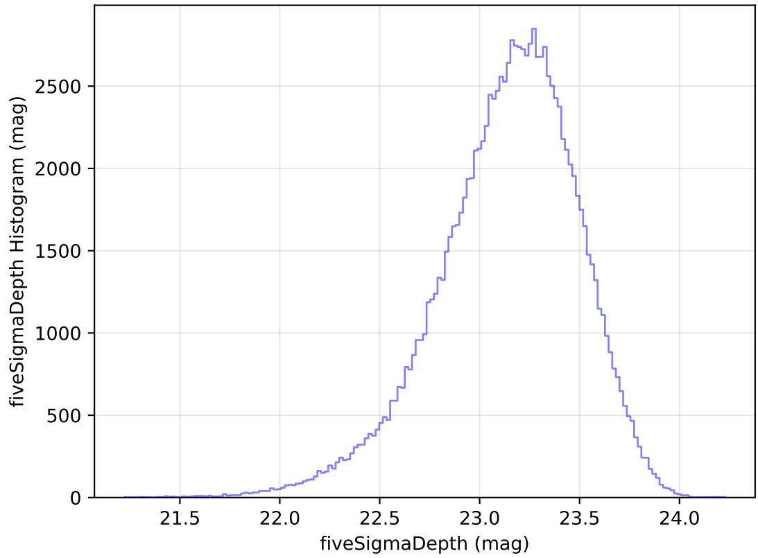
too_elab_r8_d3_ugrizy_v3.4_10yrs WFD u band: fiveSigmaDepth Histogram
