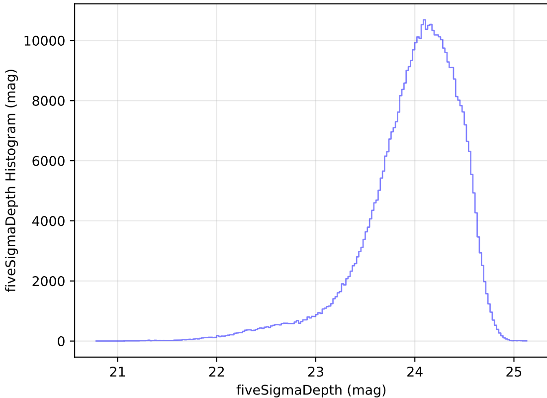
too_elab_r8_d3_ugrizy_v3.4_10yrs WFD r band: fiveSigmaDepth Histogram
