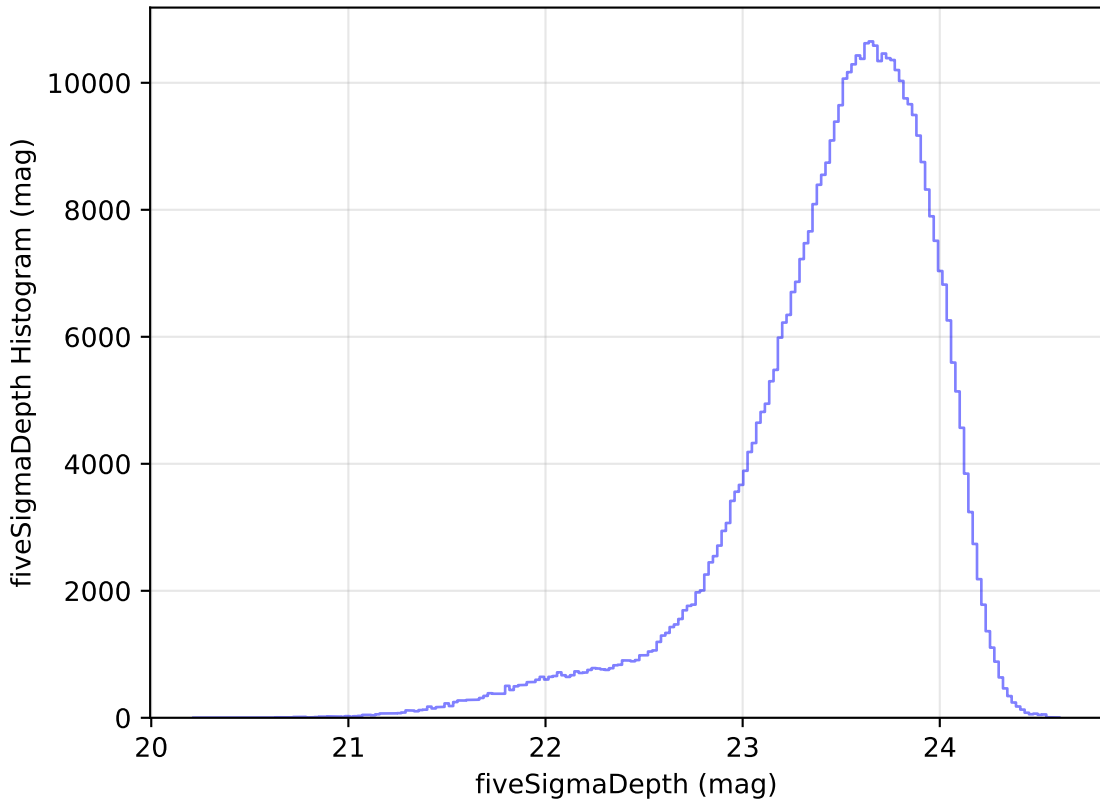
too_elab_r8_d3_ugrizy_v3.4_10yrs WFD i band: fiveSigmaDepth Histogram
