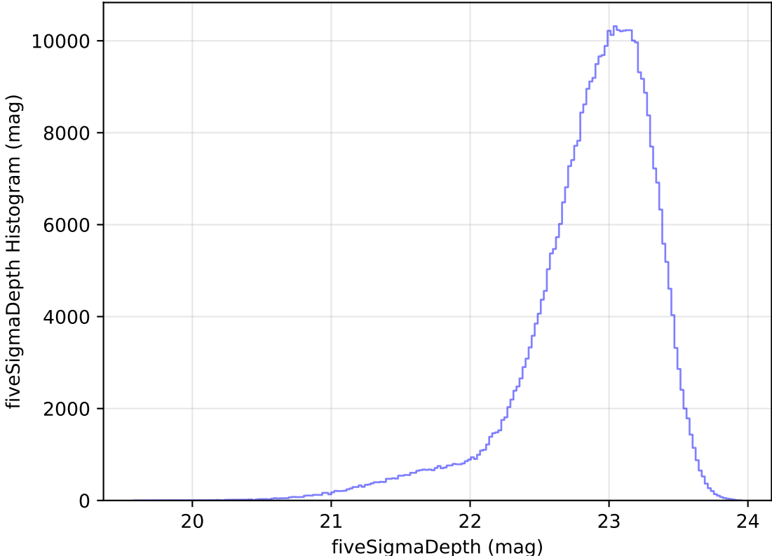
too_elab_r8_d3_ugrizy_v3.4_10yrs All sky z band: fiveSigmaDepth Histogram
