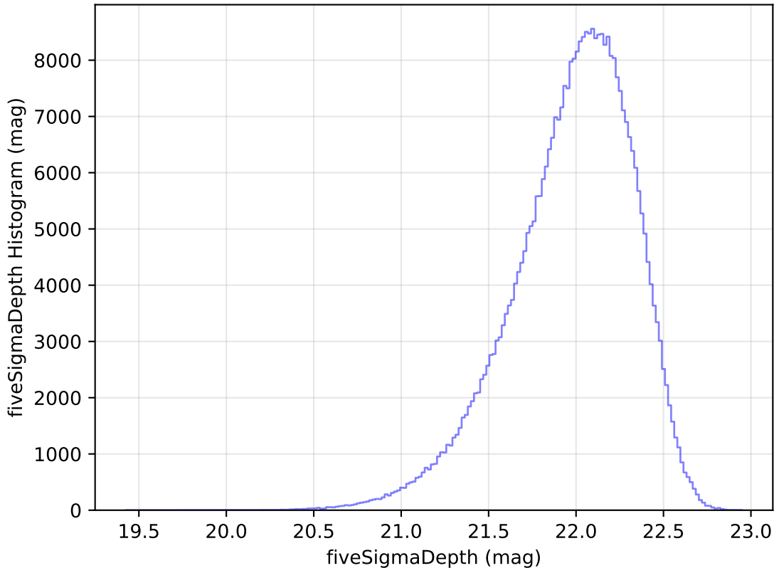
too_elab_r8_d3_ugrizy_v3.4_10yrs All sky y band: fiveSigmaDepth Histogram
