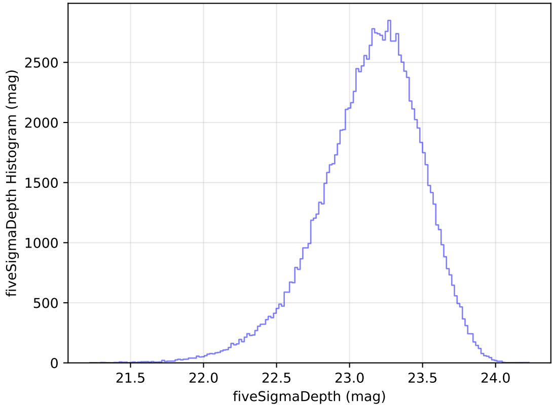
too_elab_r8_d3_ugrizy_v3.4_10yrs All sky u band: fiveSigmaDepth Histogram
