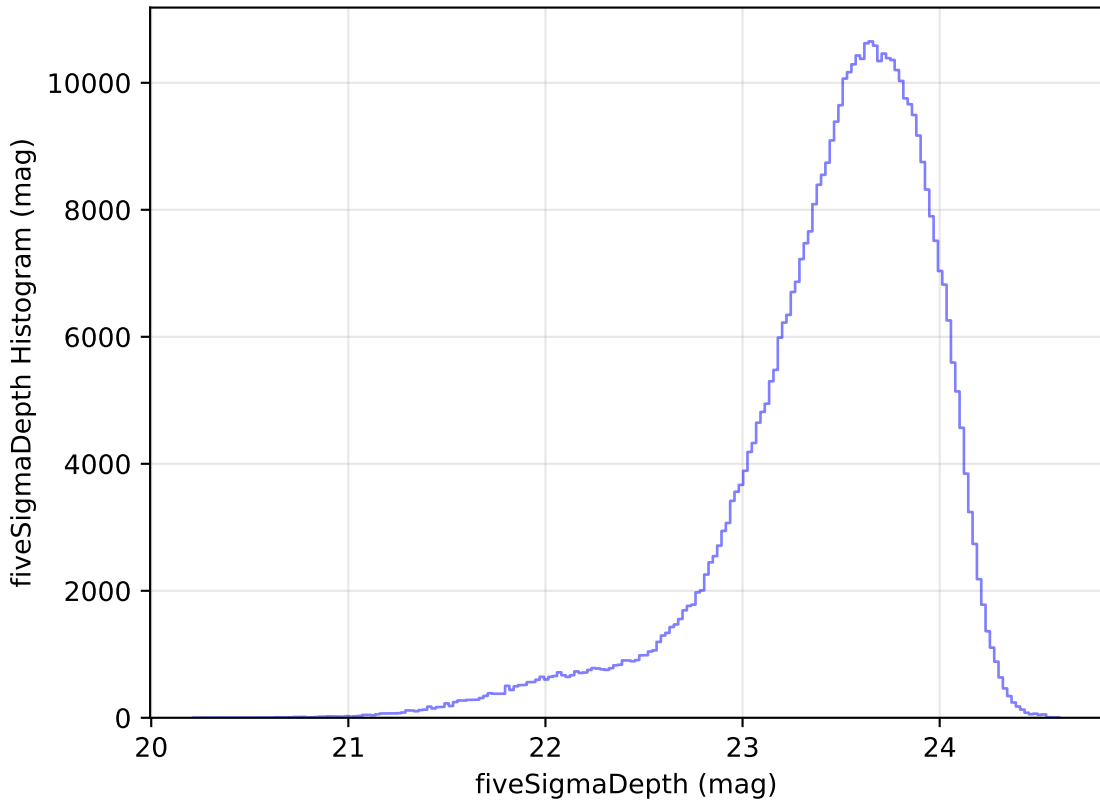
too_elab_r8_d3_ugrizy_v3.4_10yrs All sky i band: fiveSigmaDepth Histogram
