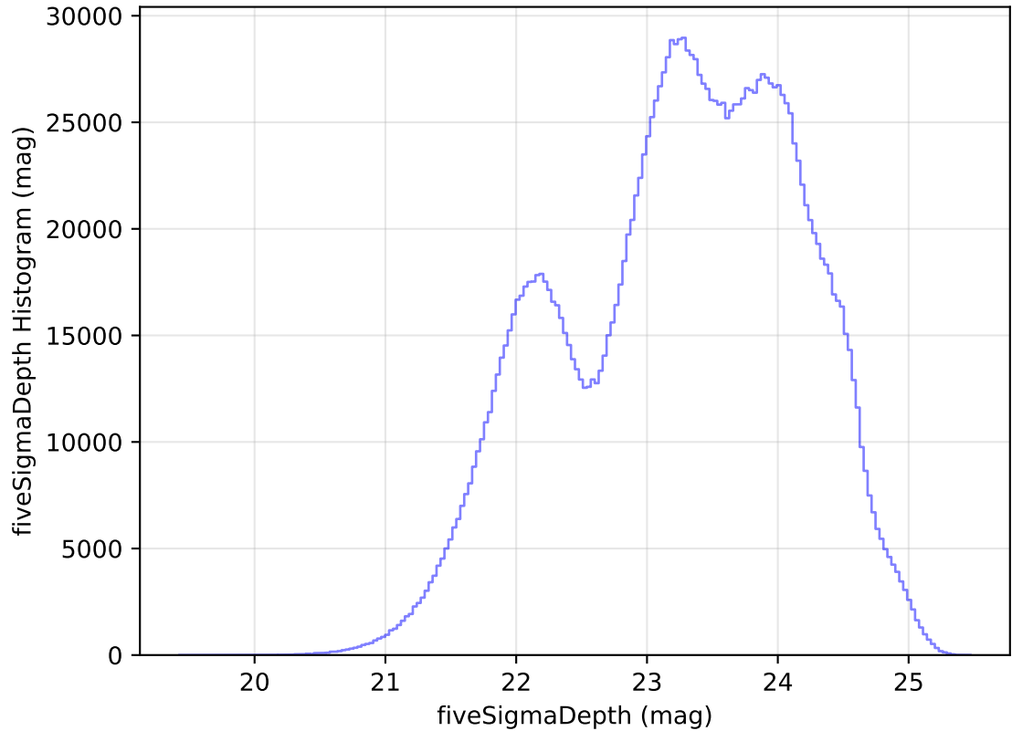
too_elab_r8_d3_ugrizy_v3.4_10yrs All sky all bands: fiveSigmaDepth Histogram
