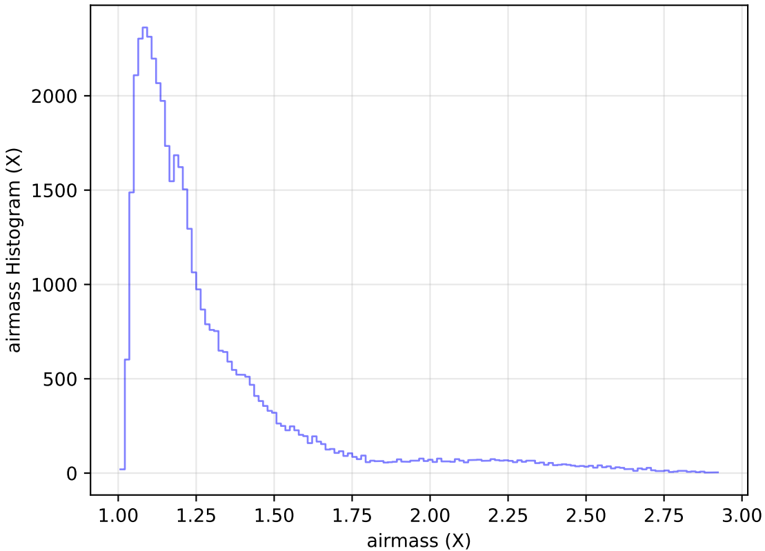
too_elab_r8_d3_ugrizy_v3.4_10yrs Yr 1 z band: airmass Histogram
