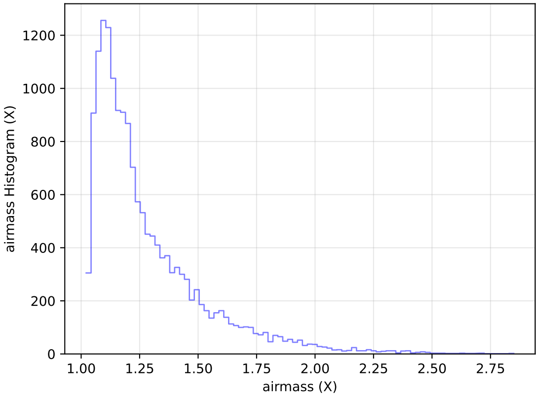
too_elab_r8_d3_ugrizy_v3.4_10yrs Yr 1 u band: airmass Histogram
