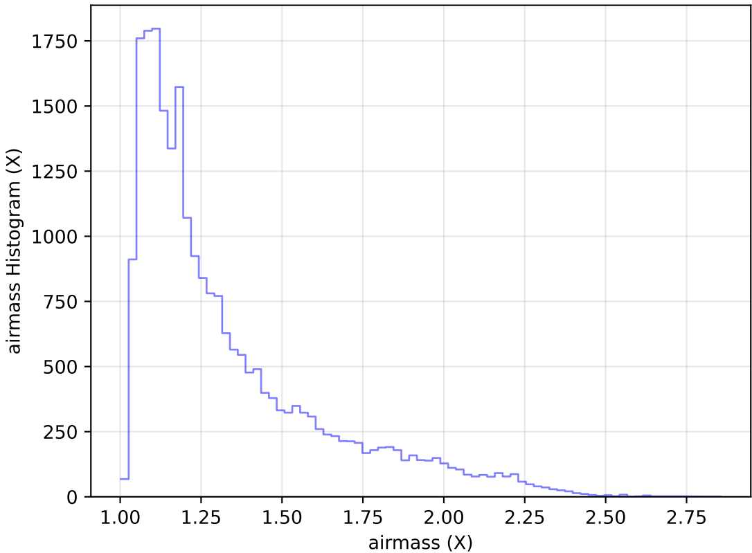
too_elab_r8_d3_ugrizy_v3.4_10yrs Yr 1 g band: airmass Histogram
