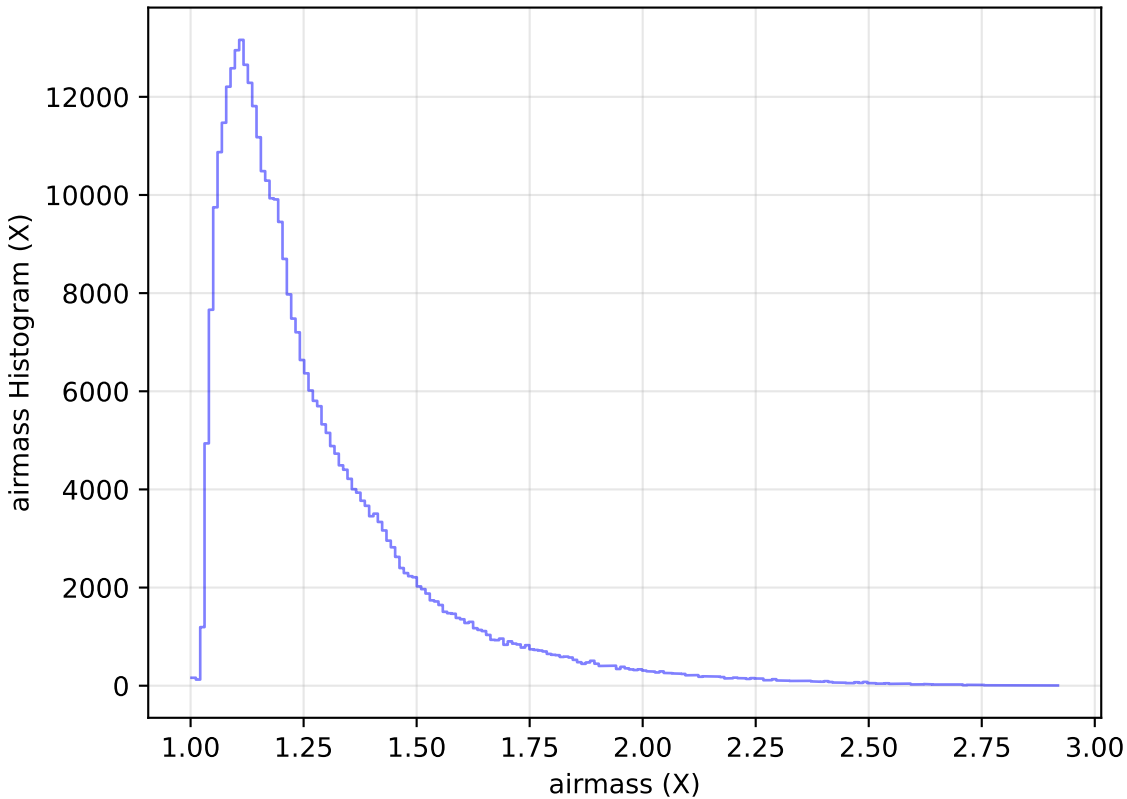
too_elab_r8_d3_ugrizy_v3.4_10yrs WFD y band: airmass Histogram
