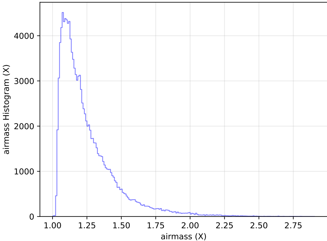
too_elab_r8_d3_ugrizy_v3.4_10yrs WFD u band: airmass Histogram
