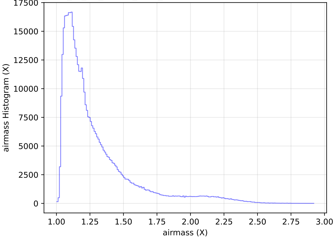
too_elab_r8_d3_ugrizy_v3.4_10yrs WFD r band: airmass Histogram
