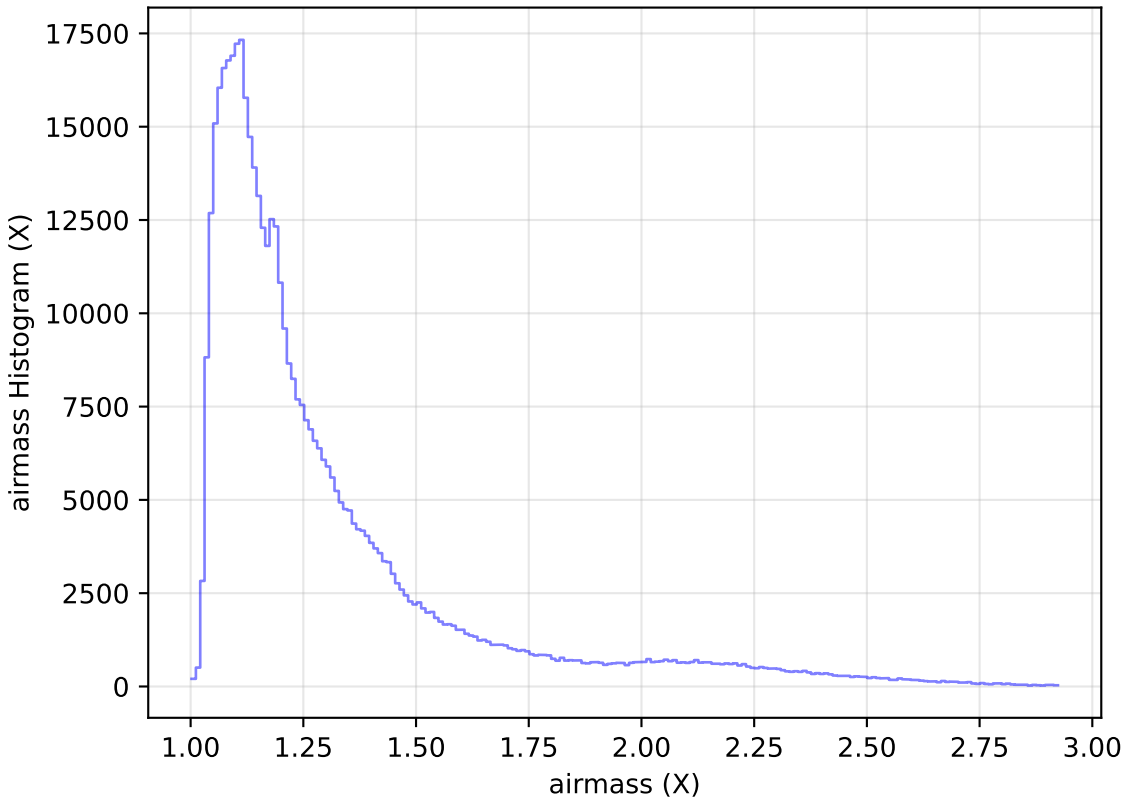
too_elab_r8_d3_ugrizy_v3.4_10yrs WFD i band: airmass Histogram
