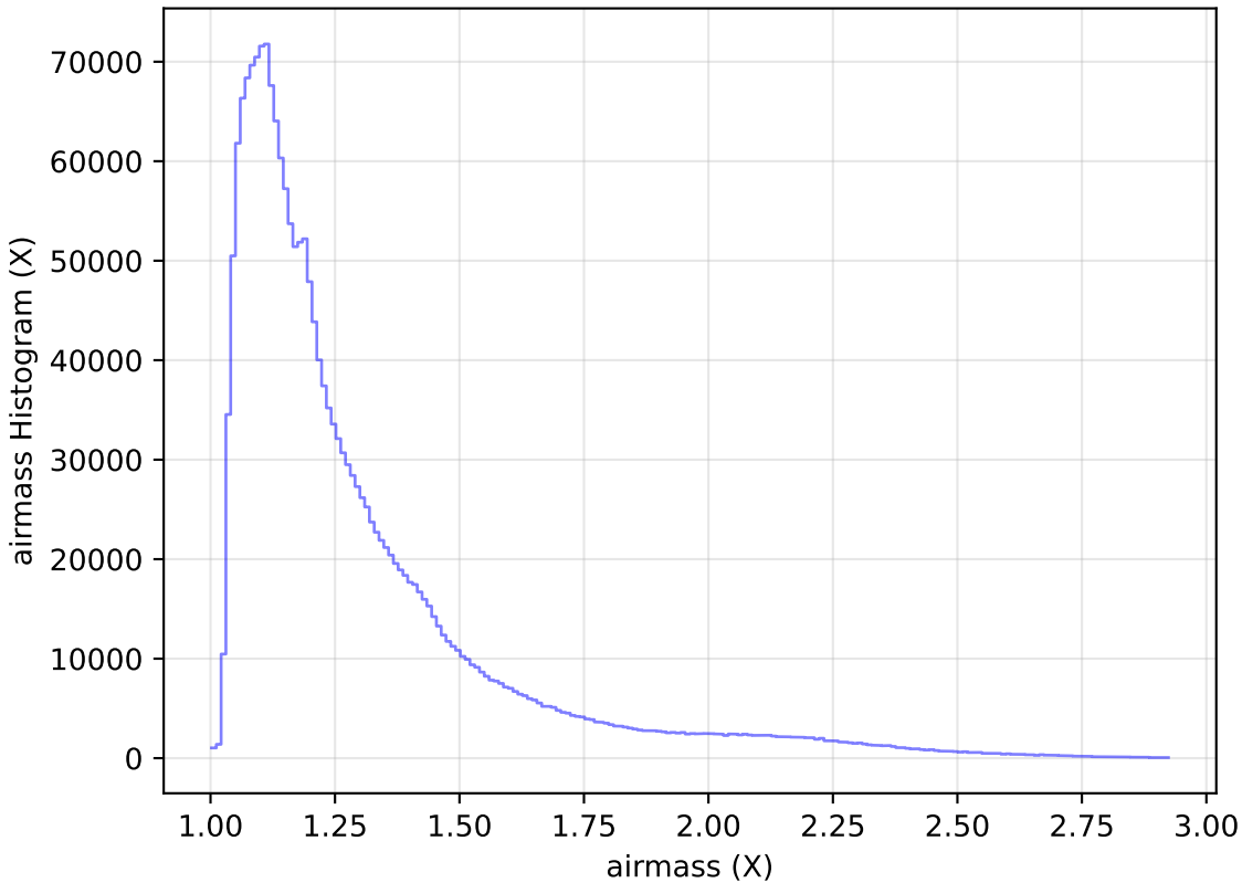
too_elab_r8_d3_ugrizy_v3.4_10yrs WFD all bands: airmass Histogram
