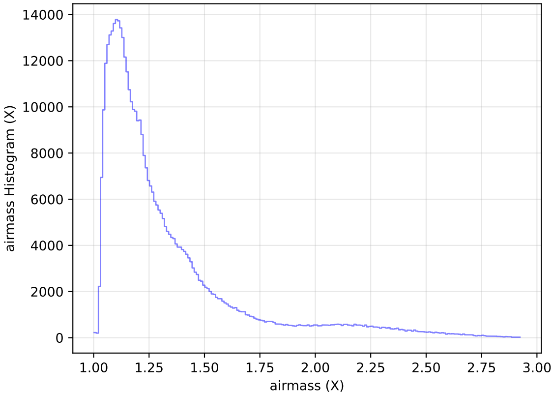
too_elab_r8_d3_ugrizy_v3.4_10yrs All sky z band: airmass Histogram
