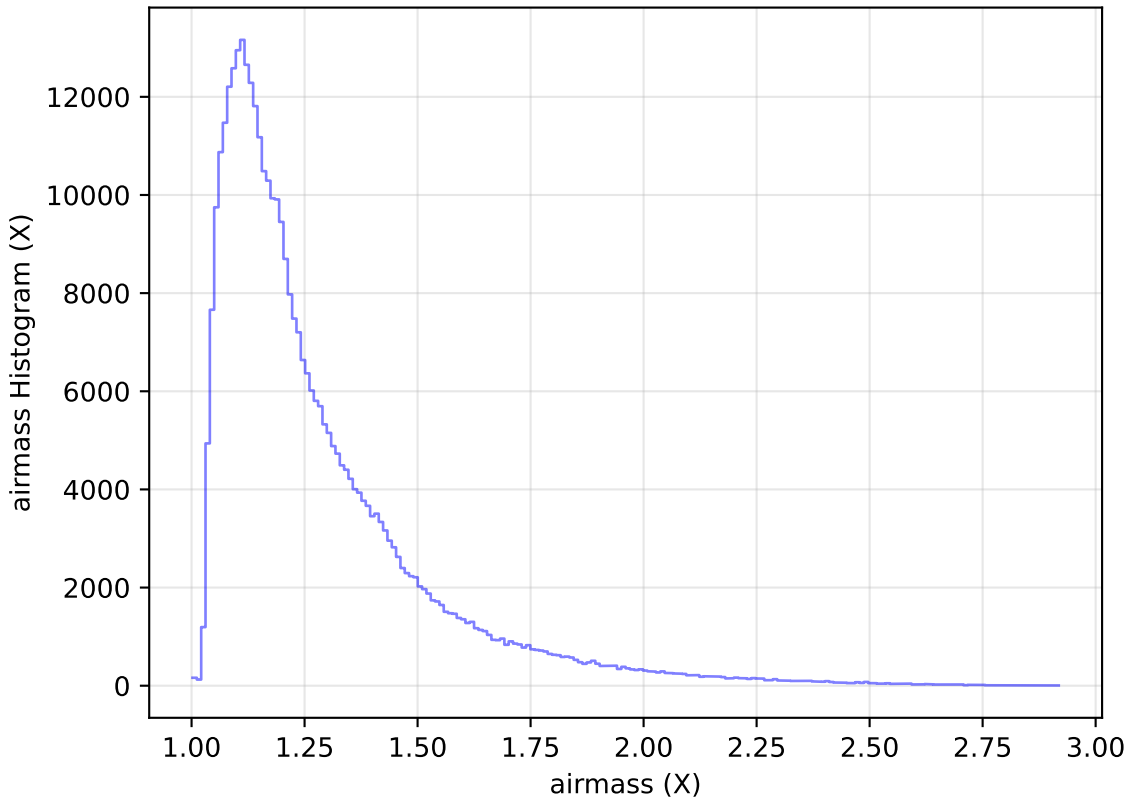
too_elab_r8_d3_ugrizy_v3.4_10yrs All sky y band: airmass Histogram
